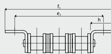
Triplex chains
