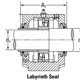
Labyrinth Seal
