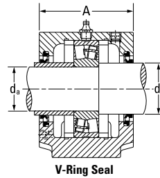
V-Ring Seal
