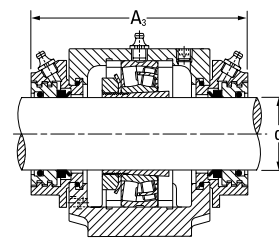
Tacanite Seal
