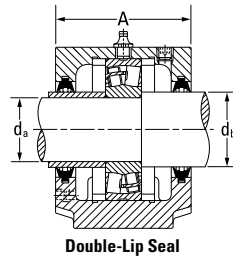
Double-Lip Seal
